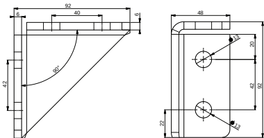
PART No. DM C6658 1 292 For Rail: Strut a 90 Pack 25
